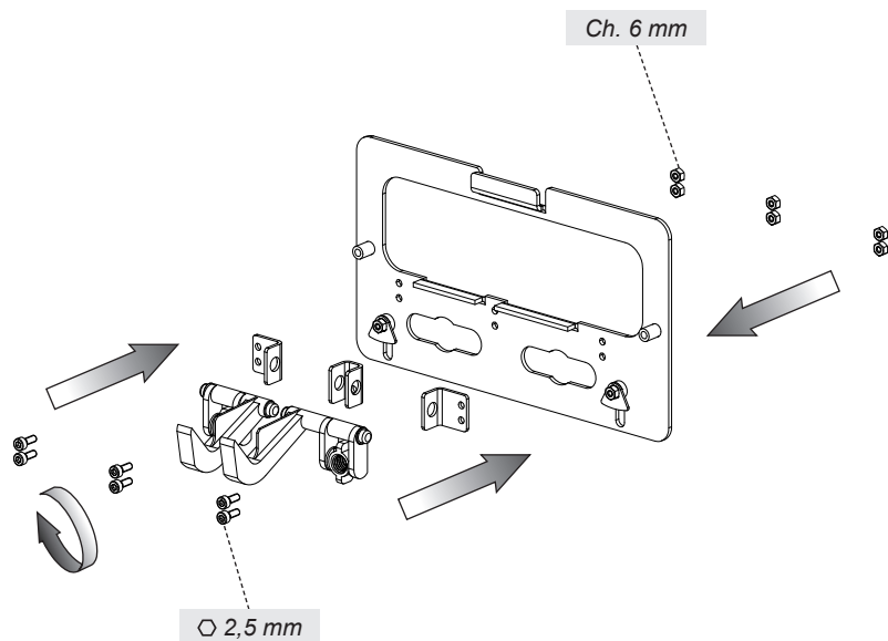
Fig. 4b - KIT DUAL FLUSH CISTERN UNI
