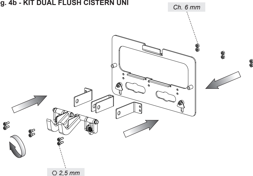
Fig. 4b - KIT DUAL FLUSH CISTERN UNI
