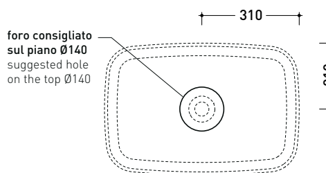
310 210 vista zenitale / zenital view
