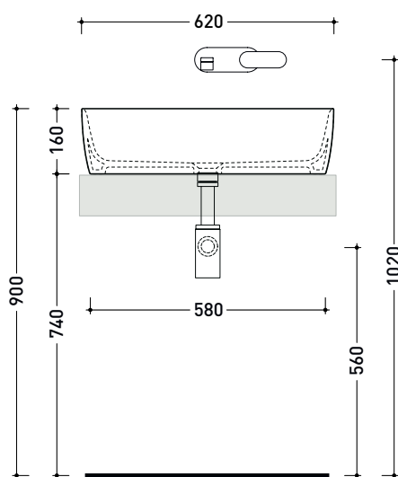
560 1020 vista frontale / frontal view
