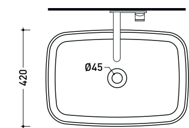
620 vista zenitale / zenital view
