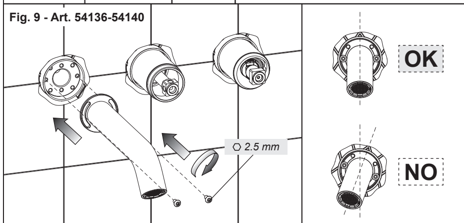
Fig. 9 - Art. 54038-54039-54239
